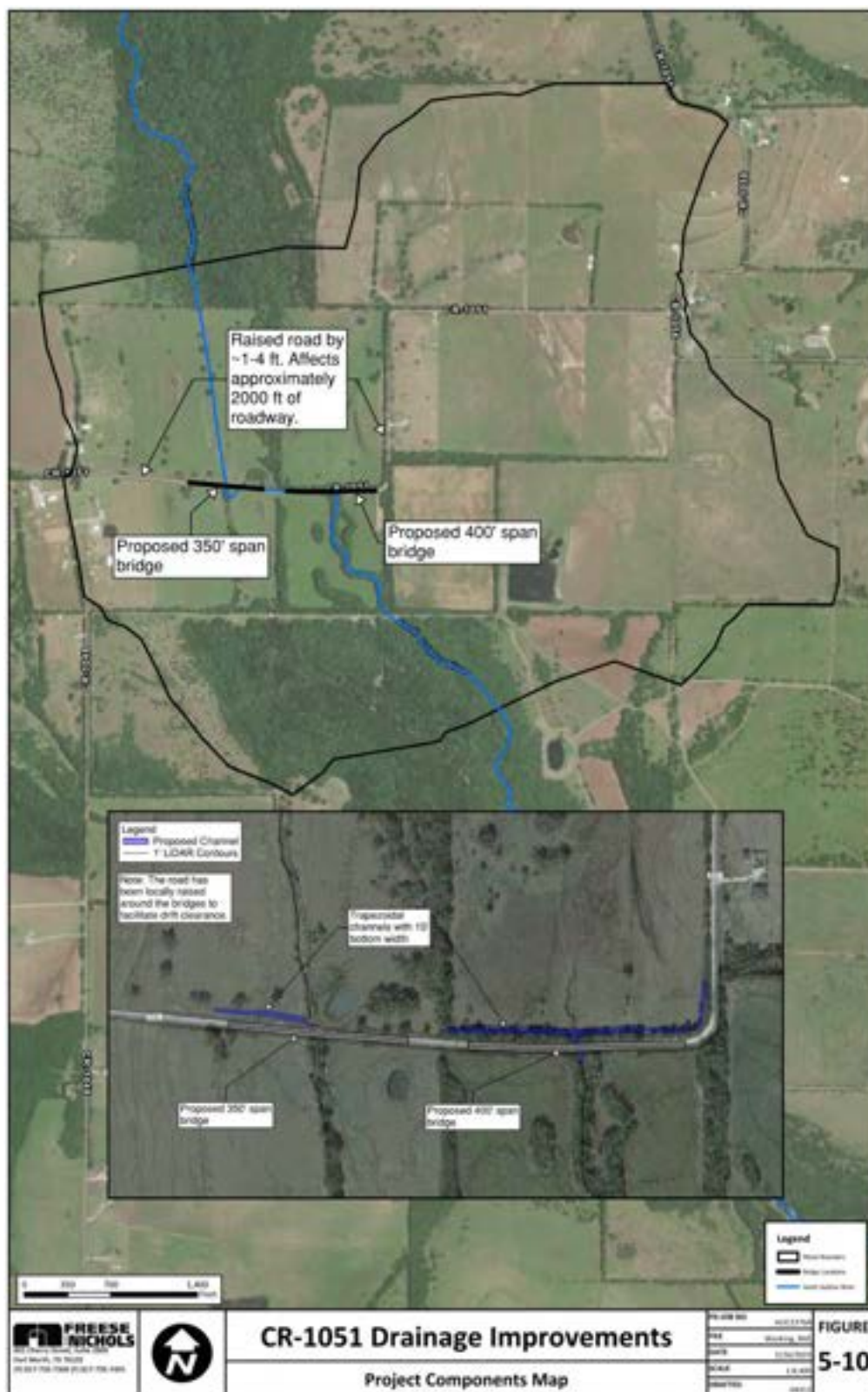
Figure 5.10 CR-1051 Drainage Improvements – Project Components (FMP 023000014)
