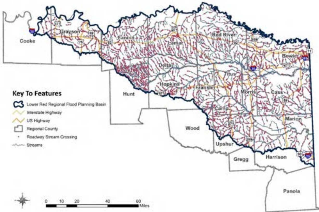
Figure 2.21 Road and Stream Crossings in the Flood Hazard Area
