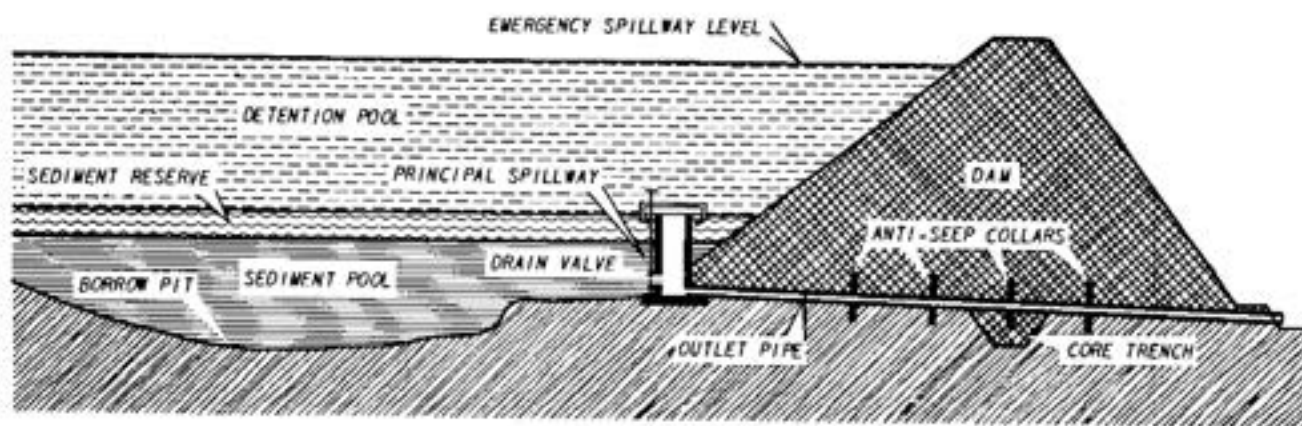
Figure 2.36 Section of a Typical NRCS Floodwater Retarding Structure (Auds Creek Watershed Work Plan, SCS, 1975)
