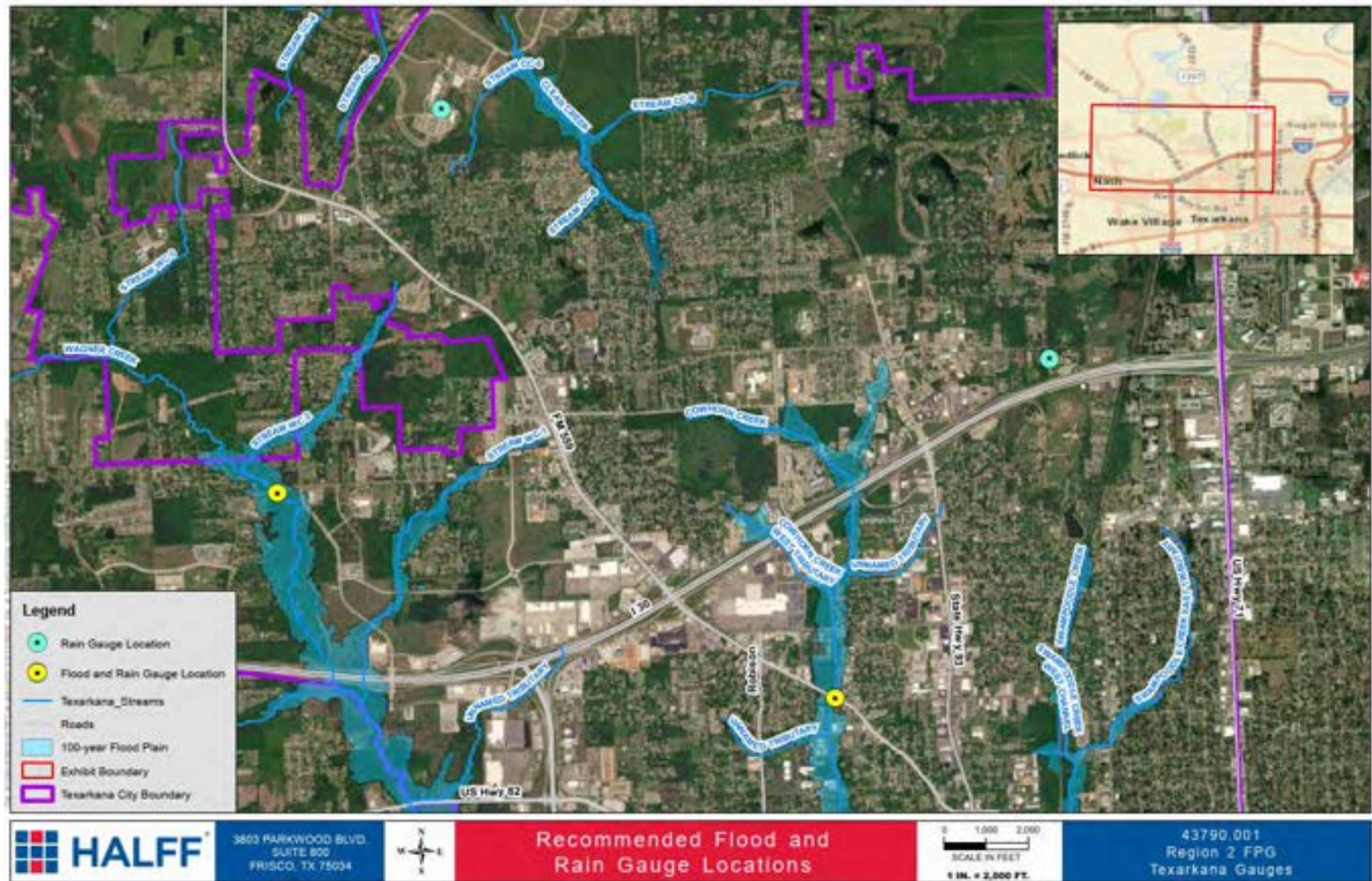
Figure 5.8 City of Texarkana Gauges – Project Components (FMP 023000011) – North Side
